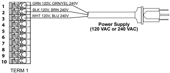
Figure 11 P110 AC Power & Relay Output Wiring
