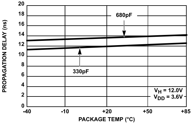
FIGURE 18. t_{pdR} vs TEMPERATURE
