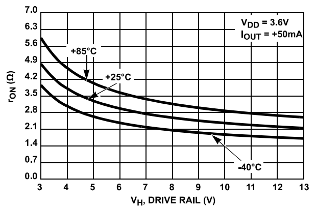
FIGURE 5. DRIVER r_{ON} vs V_H VOLTAGE (SINKING CURRENT)
