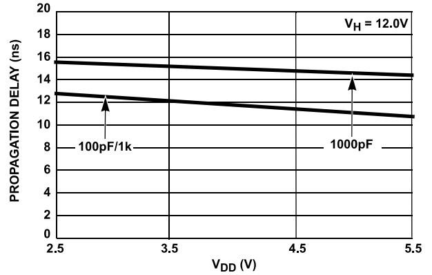
FIGURE 25. t_{pdF} vs V_{DD}
