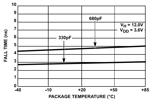
FIGURE 17. t F vs TEMPERATURE
